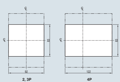
Front panel cutting
