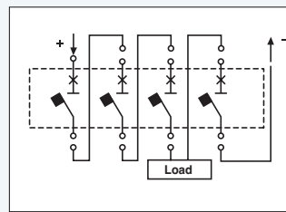
DC1000V (4P)
