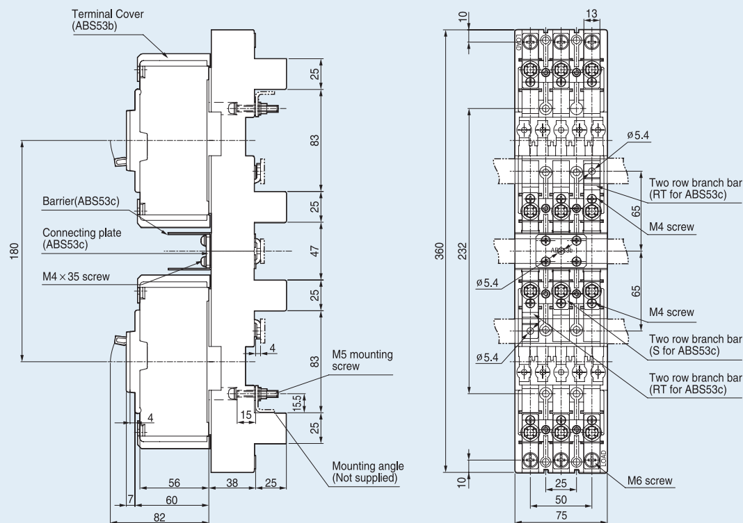
Mounting dimensions
