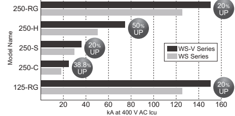
■ Breaking capacity comparison with a conventional model
