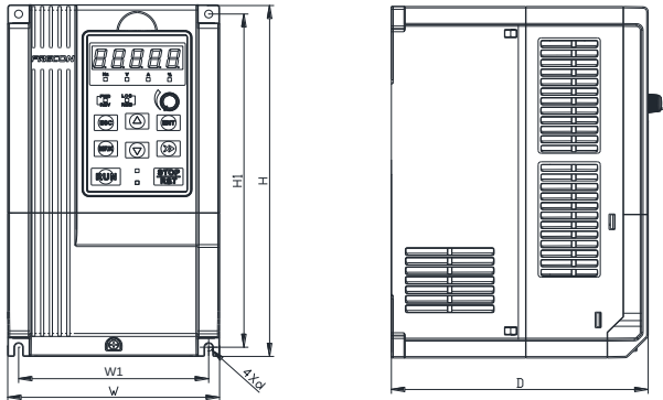
Fig 1-7 4~22kW Wall installation diagram
