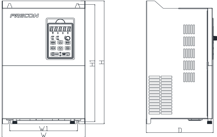
Fig 1-8 30~450kW Wall installation diagram
