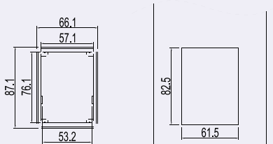
Installation bracket
