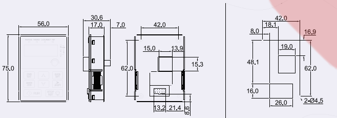
Overall drawing
